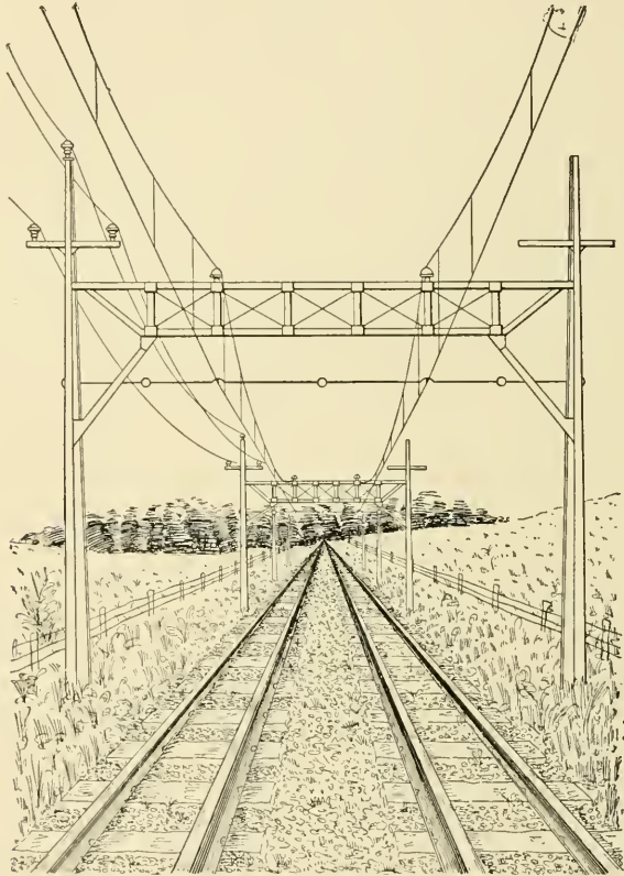
Fig. 199. Catenary System on Light Brace Construction
